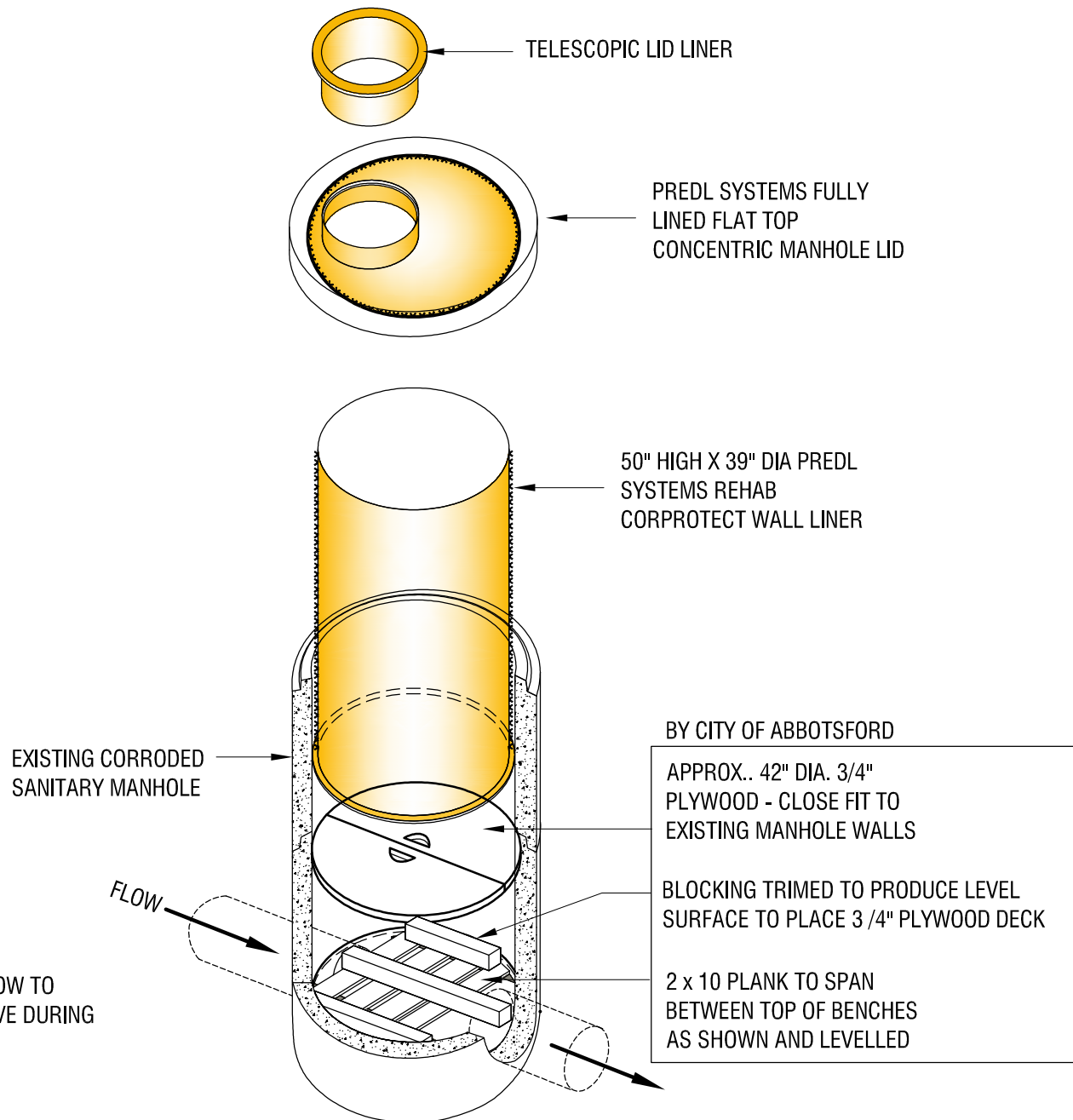
42" DIA. WALL LINER REHAB CITY OF ABBOTSFORD
